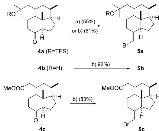
Scheme 2. Synthesis of alkenyl bromides 5a–c . TES = SiEt 3 . a) Trost conditions: Ph 3 P + CH 2 BrBr − , NaHMDs (HMDs = hexamethyldisilazane), THF; b) new conditions: Ph 3 P + CH 2 BrBr − washing with toluene/CH 2 Cl 2 under ultrasonication, then KOtBu, -15 \rightarrow 0^\circ\text{C} .
