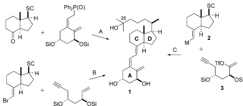
Scheme 1. Synthetic routes to vitamin D compounds. M = metal, SC = side chain, Si = protecting group.
