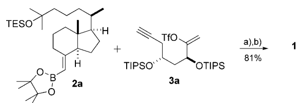
Scheme 3. Synthesis of the natural hormone 1 : a) [PdCl 2 (Ph 3 P) 2 ] (5 mol %), 2 M K 3 PO 4 (aq)/THF, RT, 1 h; b) n Bu 4 NF, THF, RT, 24 h. TIPS = Si( i Pr) 3 .
